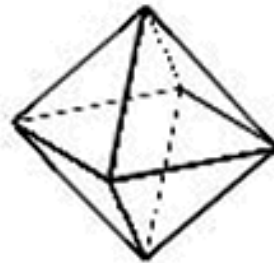
Octahedron
