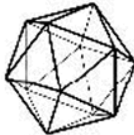
Icosahedron
